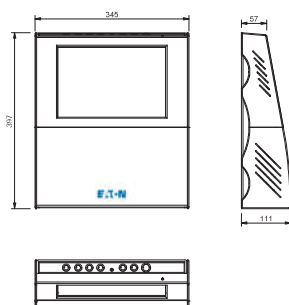
Dimensional drawing Controller, data in mm
